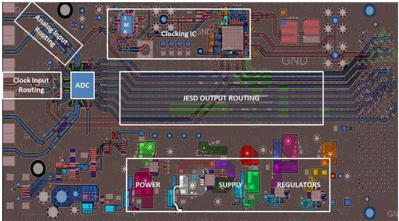
Figure 244. ADC32RF44EVM Layout
