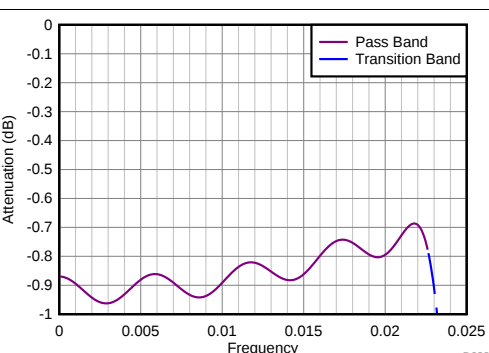
Figure 91. Divide-by-18 Filter Response (Zoomed)
