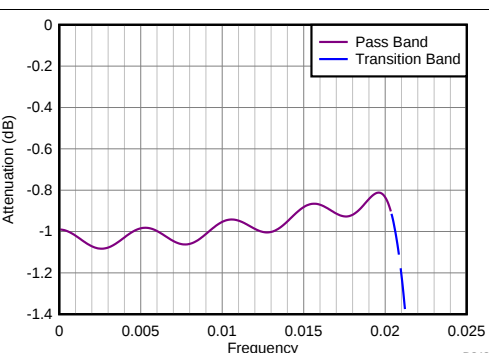
Figure 93. Divide-by-20 Filter Response (Zoomed)
