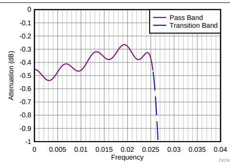
Figure 89. Divide-by-16 Filter Response (Zoomed)
