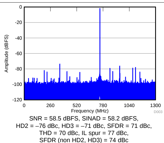
Figure 242. FFT for 1850-MHz Input Frequency
