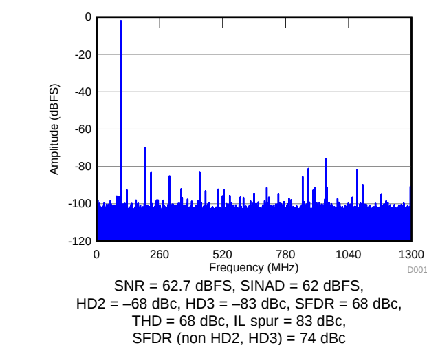
Figure 241. FFT for 100-MHz Input Frequency
