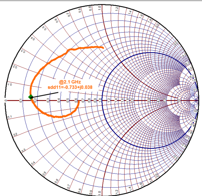
Figure 59. SDD11 Over the Input Frequency Range
