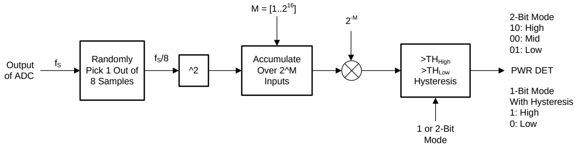
Figure 74. RMS Power Detector Implementation
