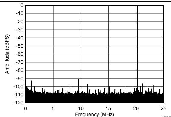
SFDR = 89.7 dBc, SFDR = 93 dBc (non 23), SNR = 72.9 dBFS, SINAD = 72.8 dBFS, THD = 86.6 dBc, HD2 = -89.7 dBc, HD3 = -107.7 dBc
