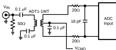
Figure 19. Low Input Frequency Transformer Drive Circuit
