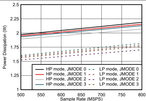
Figure 5-74. Quad Channel, Power Dissipation vs F_S for JMODES 0 - 3
