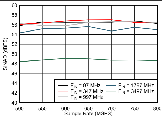
Figure 5-30. SINAD vs Sample Rate
