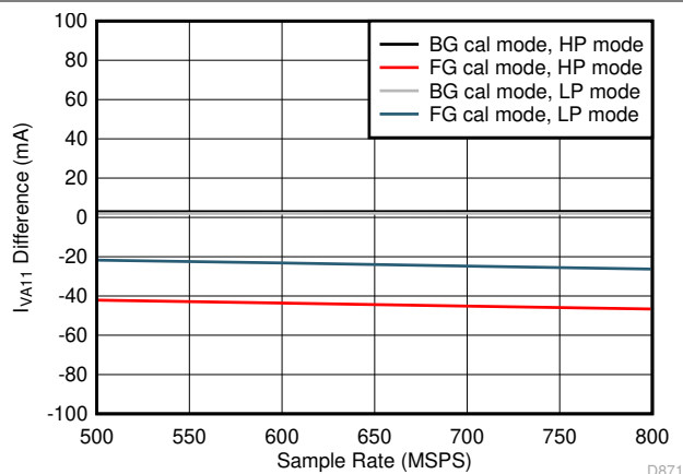
Figure 5-86. Quad Channel, I_{VA11} vs F_S over Modes
