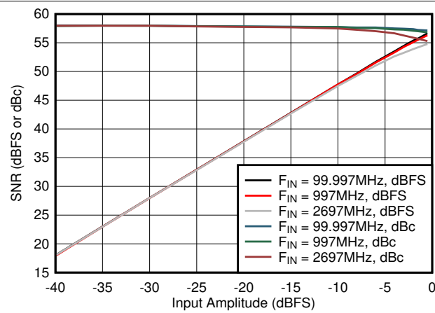
Figure 5-32. SNR vs Input Amplitude
