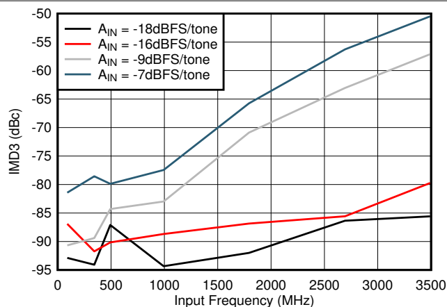
Figure 5-72. IMD3 vs Input Frequency
