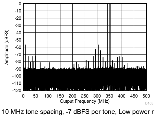
Figure 6-72. Two Tone FFT at 348 MHz
