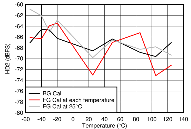
Figure 5-66. HD2 vs Temperature
