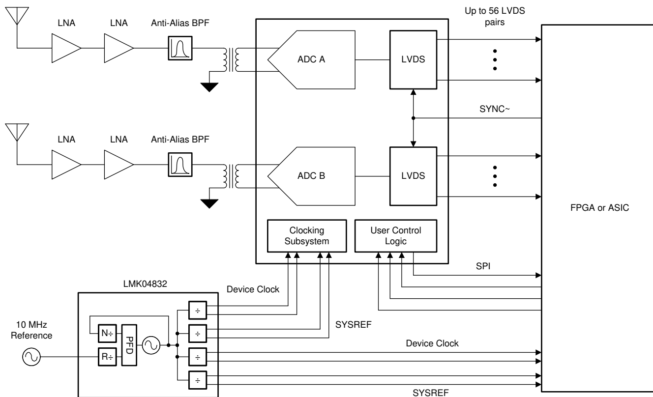
Figure 8-1. Typical Configuration for Wideband RF Sampling
