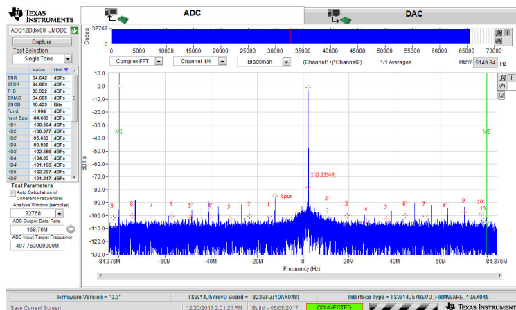
Figure 7-4. FFT for 497.77MHz Input Signal, 2.7 SPS, Decimation-by-16, f_{NCO} = 500 MHz, JMODE16
