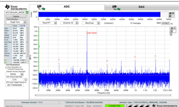
Figure 7-3. FFT for 497.77MHz Input Signal, 2.7GSPS, JMODE2
