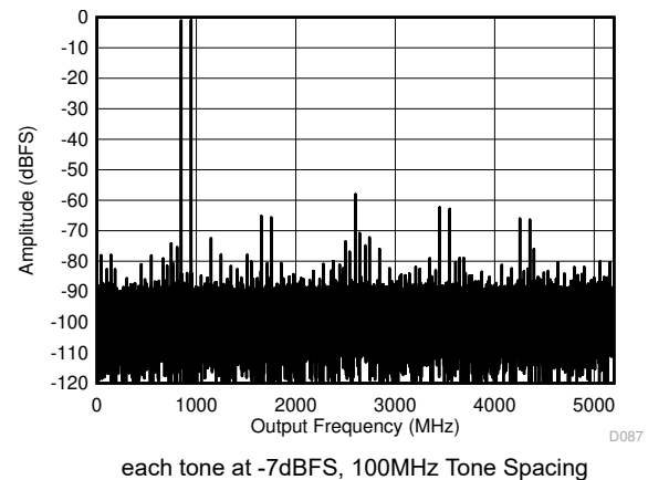
Figure 5-12. DES Mode: Two Tone FFT at 897MHz
