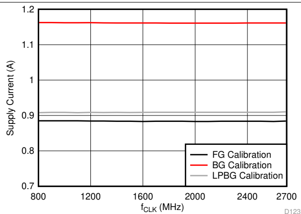
Figure 53. IA19 Supply Current vs Clock Frequency
