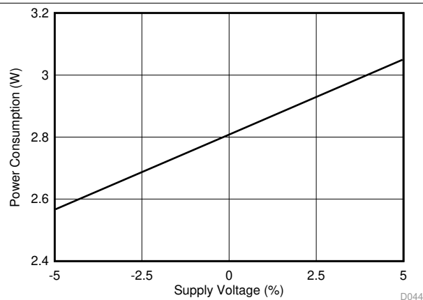
Figure 52. Power Consumption vs Supply Voltage
