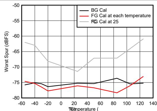
Figure 5-68. Worst Spur vs Temperature
