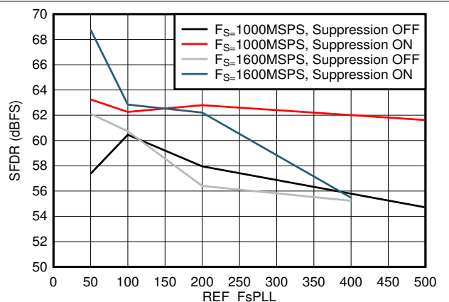
Figure 5-39. SFDR vs F_{REF} and Suppression
