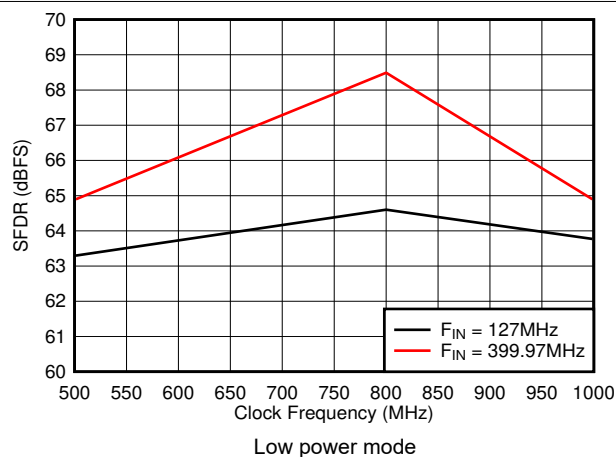
Figure 5-29. SFDR vs Sample Rate
