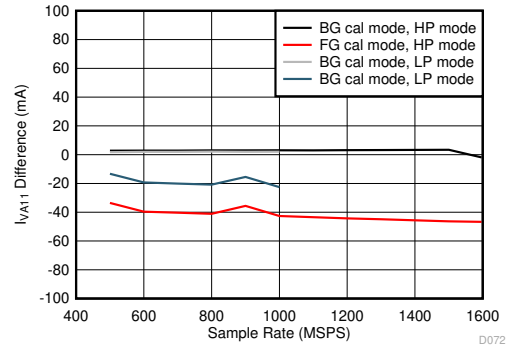
Figure 5-116. Dual Channel, I_{VA11} Change with Calibration Mode
