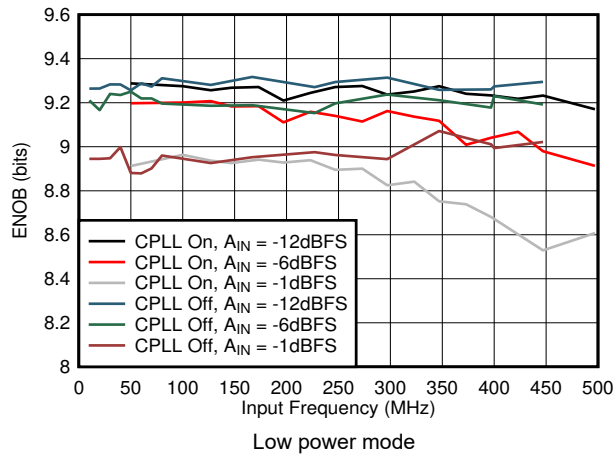
Figure 5-57. ENOB vs A_{IN} and C-PLL
