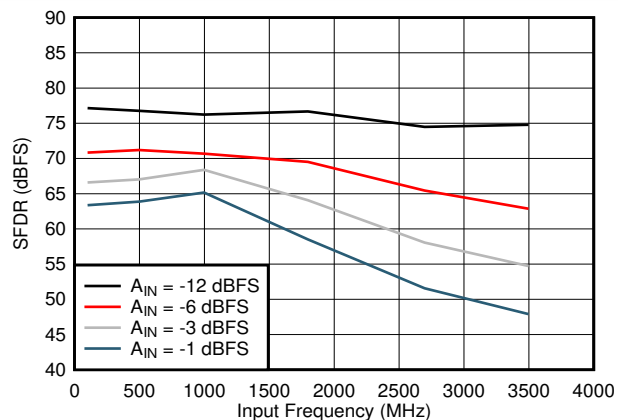
Figure 5-17. SFDR vs Input Frequency
