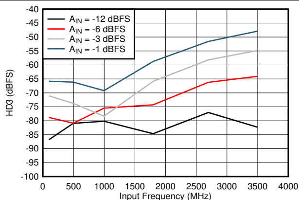
Figure 5-22. HD3 vs Input Frequency
