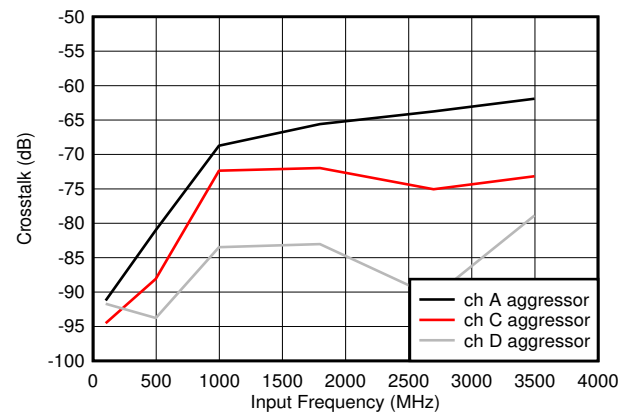
Figure 5-78. Crosstalk to Channel B vs F_{IN}
