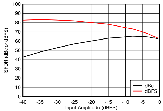
Figure 5-34. SFDR vs A_{IN}
