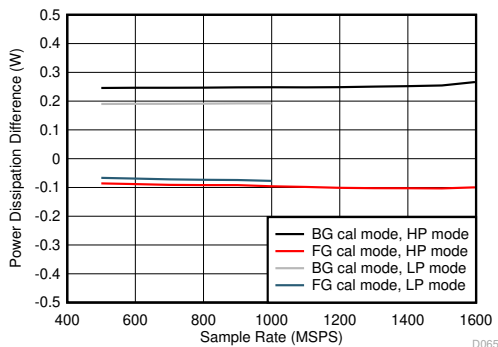
Figure 5-109. Quad Channel, Power Dissipation Change with Calibration Mode
