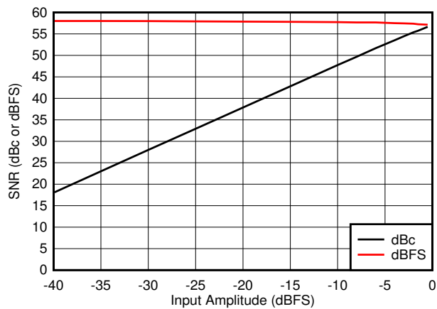
Figure 5-35. SNR vs A_{IN}
