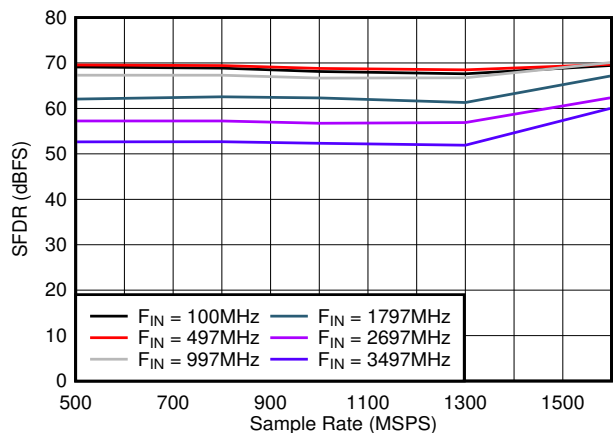
Figure 5-23. SFDR vs Sample Rate
