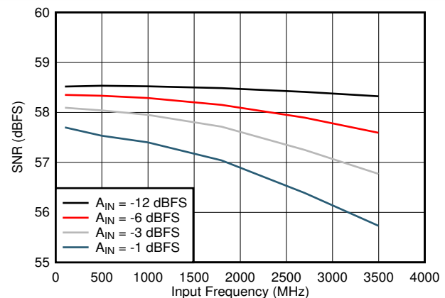
Figure 5-18. SNR vs Input Frequency
