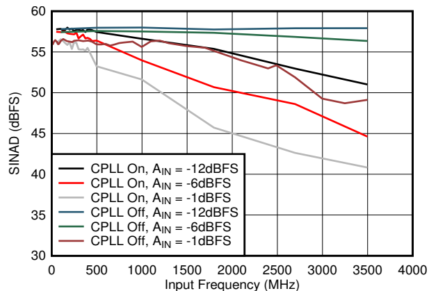
Figure 5-50. SINAD vs A_{IN} and C-PLL
