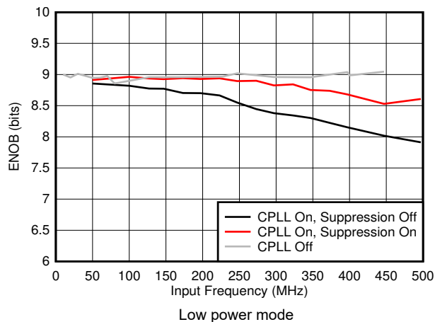
Figure 5-47. ENOB vs F_{IN} and C-PLL modes
