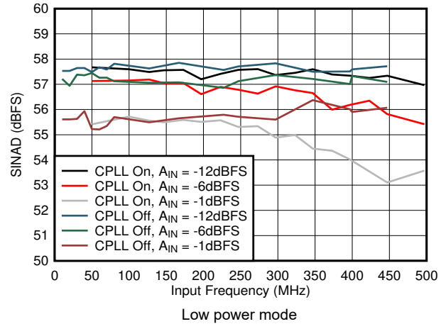
Figure 5-56. SINAD vs A_{IN} and C-PLL
