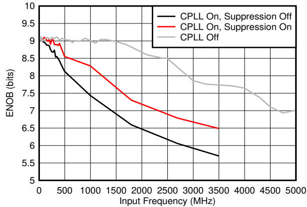
Figure 5-43. ENOB vs F_{IN} and C-PLL modes
