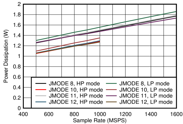
Figure 5-91. Dual Channel, Power Dissipation vs F_s and JMODE 8 - 12
