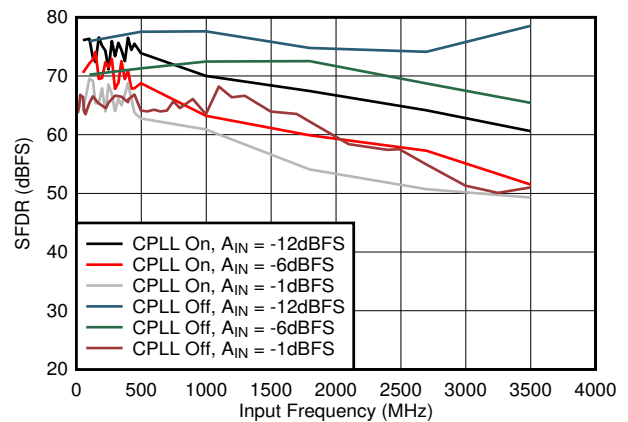
Figure 5-48. SFDR vs A_{IN} and C-PLL
