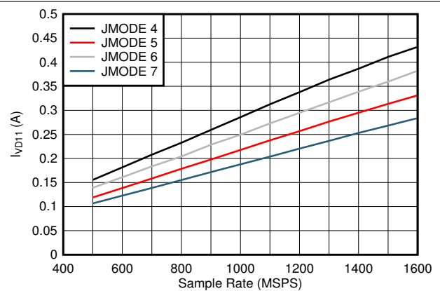
Figure 5-94. Dual Channel, I_{VD11} vs F_s
