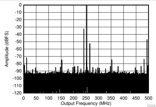
Figure 5-14. Single Tone FFT at 897MHz and -1dBFS
