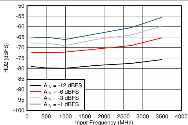
Figure 5-21. HD2 vs Input Frequency
