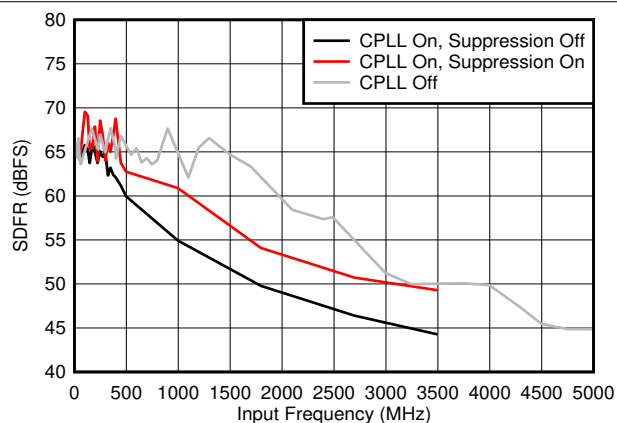
Figure 5-40. SFDR vs F_{IN} and C-PLL modes
