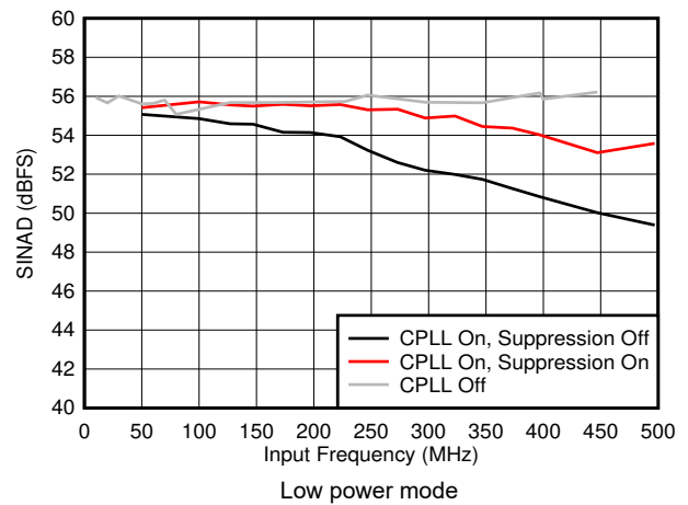
Figure 5-46. SINAD vs F_{IN} and C-PLL modes
