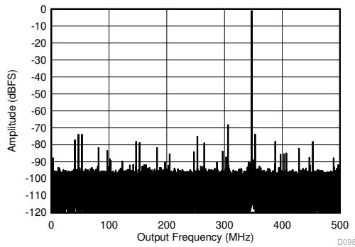
Figure 5-13. Single Tone FFT at 347MHz and -1dBFS
