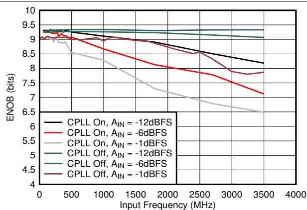
Figure 5-51. ENOB vs A_{IN} and C-PLL
