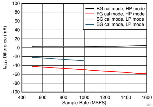
Figure 5-115. Quad Channel, I_{VA11} Change with Calibration Mode
