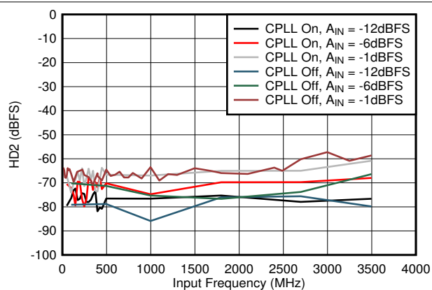
Figure 5-52. HD2 vs A_{IN} and C-PLL
