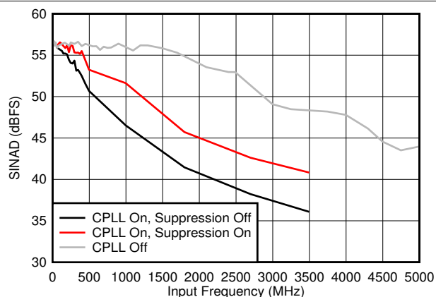
Figure 5-42. SINAD vs F_{IN} and C-PLL modes
