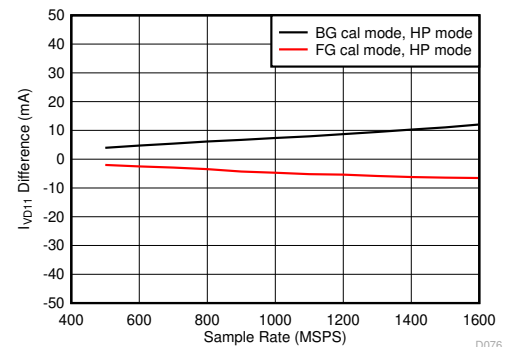
Figure 5-118. Quad Channel, I_{VD11} Change with Calibration Mode
