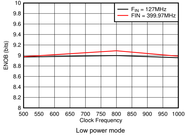
Figure 5-31. ENOB vs Sample Rate
