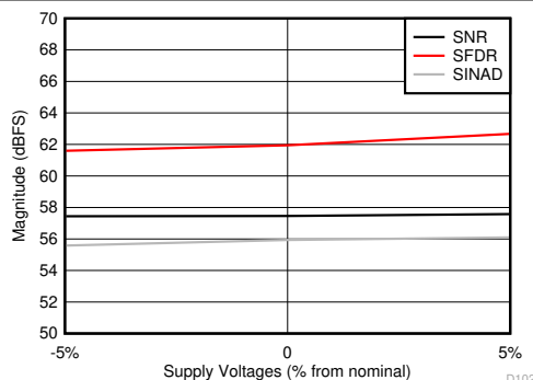
Figure 5-62. SNR, SFDR and SINAD vs Supply Voltages
