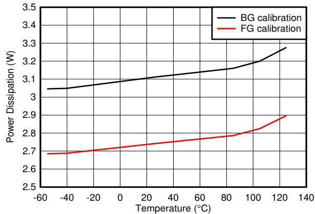
Figure 5-121. Quad Channel, Power Dissipation vs Temperature
