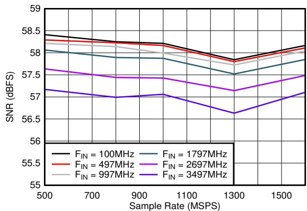
Figure 5-24. SNR vs Sample Rate
