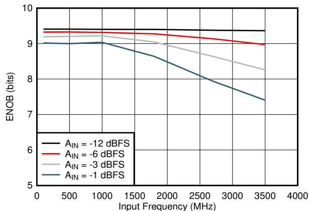
Figure 5-20. ENOB vs Input Frequency
