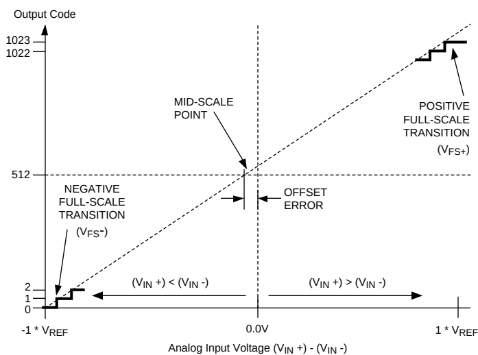
Figure 3. Transfer Characteristic
