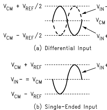
Figure 23. Expected Input Signal Range
