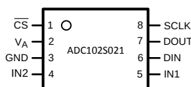
Figure 1. VSSOP Package See Package Number DGK0008A
