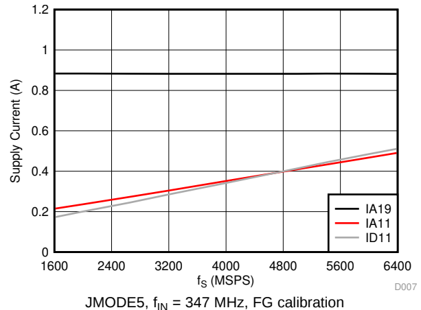
Figure 43. Supply Current vs Sampling Rate
