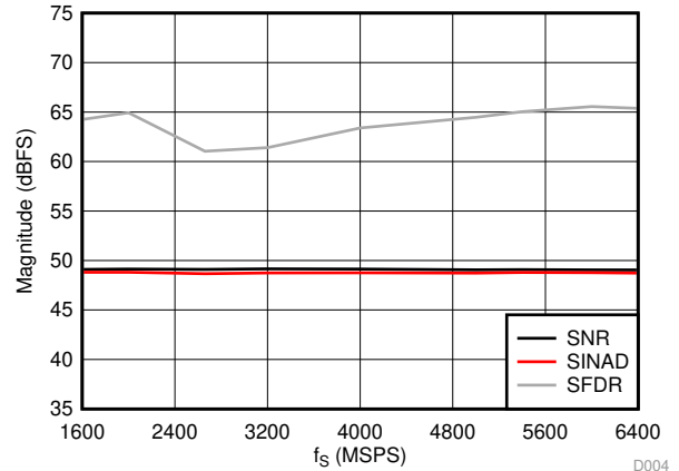
JMODE5, f_{\text{IN}} = 347\text{ MHz} , BG calibration
