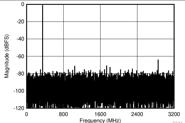
JMODE5, f_{\text{IN}} = 350\text{ MHz} , FG calibration, SNR = 49.0 dBFS, SFDR = 64.0 dBFS, ENOB = 7.80 bits
