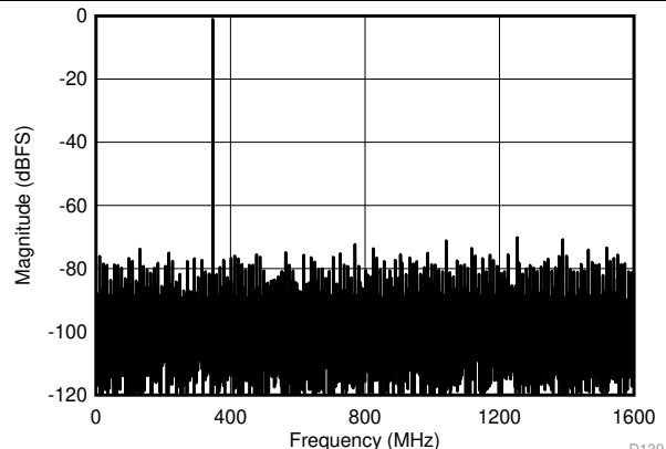
JMODE7, f_{\text{IN}} = 350\text{ MHz} , FG calibration, SNR = 49.1 dBFS, SFDR = 70.1 dBFS, ENOB = 7.80 bits
