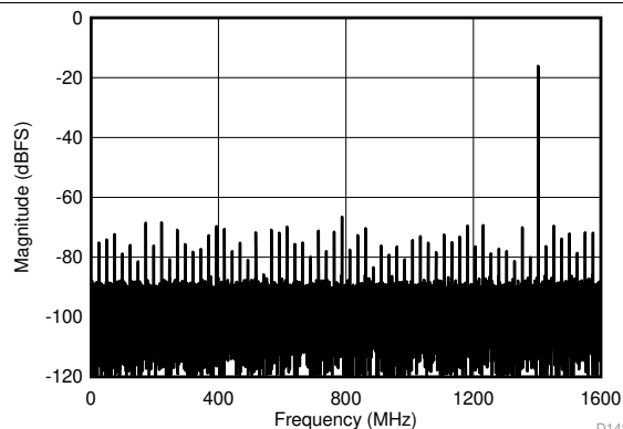
JMODE7, f_{\text{IN}} = 8200\text{ MHz} , FG calibration, SNR = 49.2 dBFS, SFDR = 65.9 dBFS, ENOB = 7.80 bits
