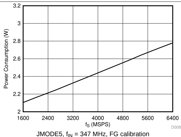
Figure 44. Power Consumption vs Sampling Rate
