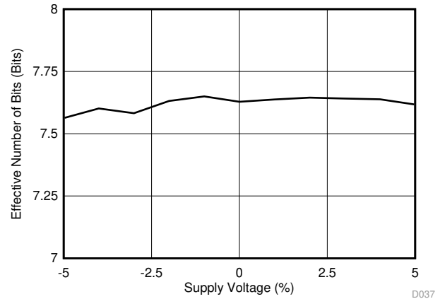
Figure 41. ENOB vs Supply Voltage
