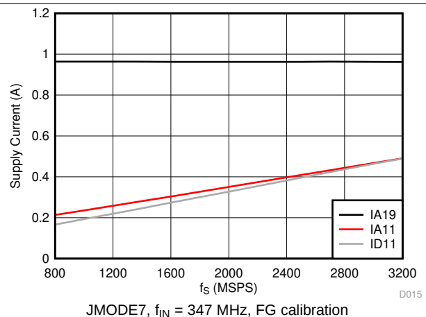
Figure 45. Supply Current vs Sampling Rate
