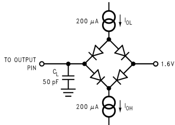
Figure 2. Timing Test Circuit
